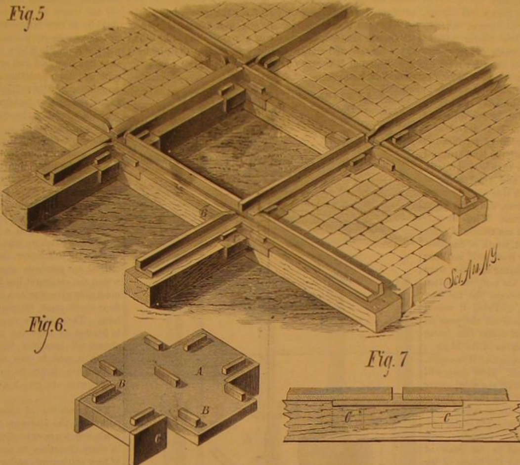
RAILWAY CROSSING.
