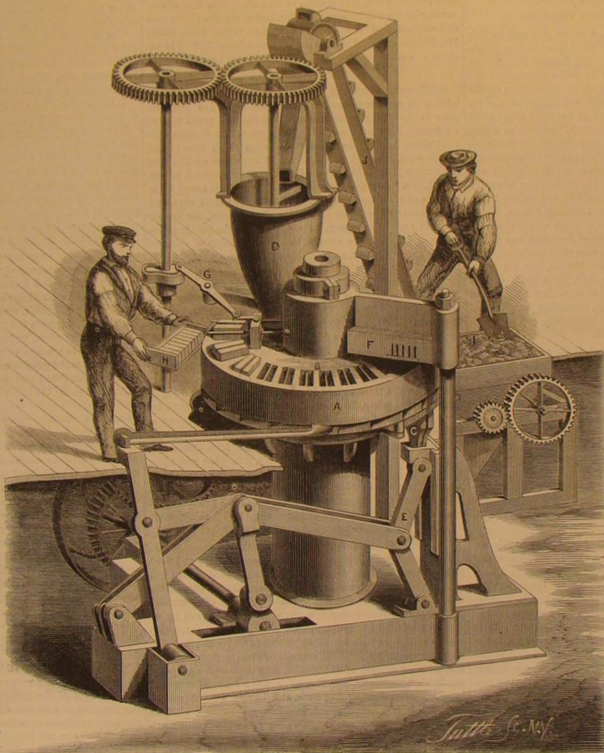
SHEPARD'S IMPROVED BRICK PRESS.
