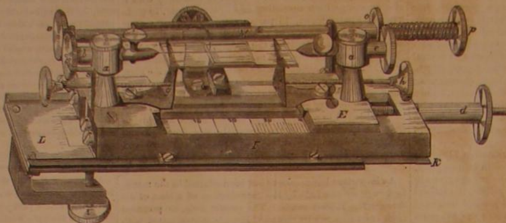
INSTRUMENT FOR MEASURING FIBERS.
