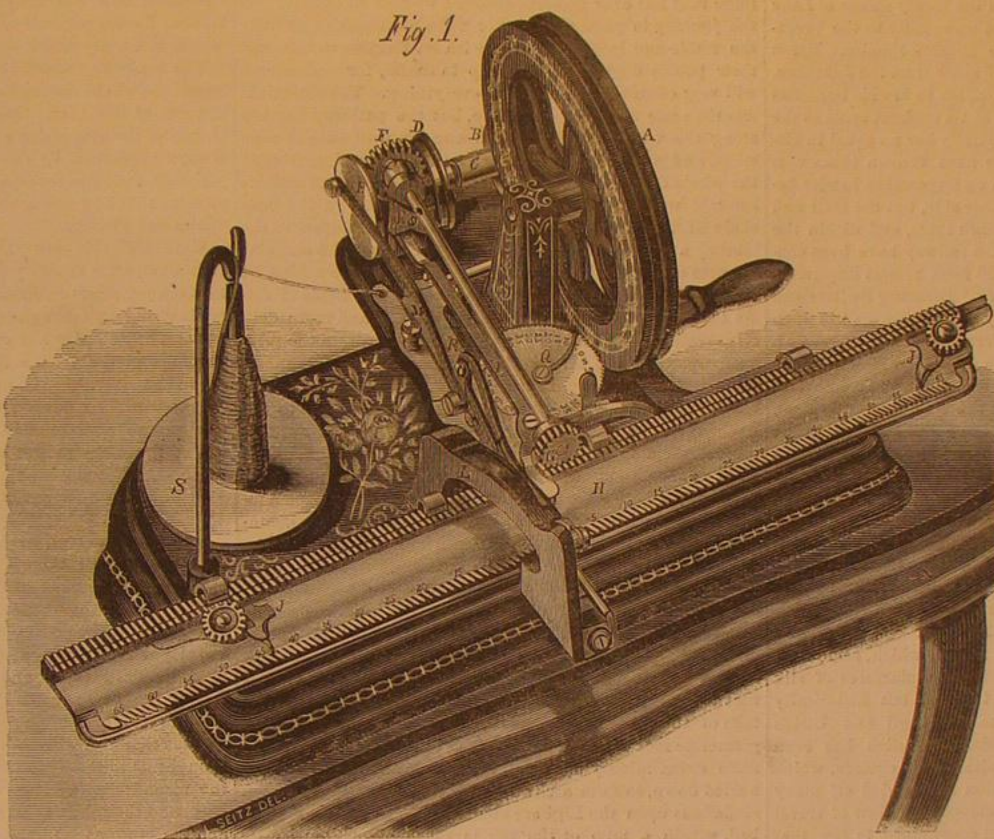
THE HINKLEY PATENT KNITTING MACHINE.
