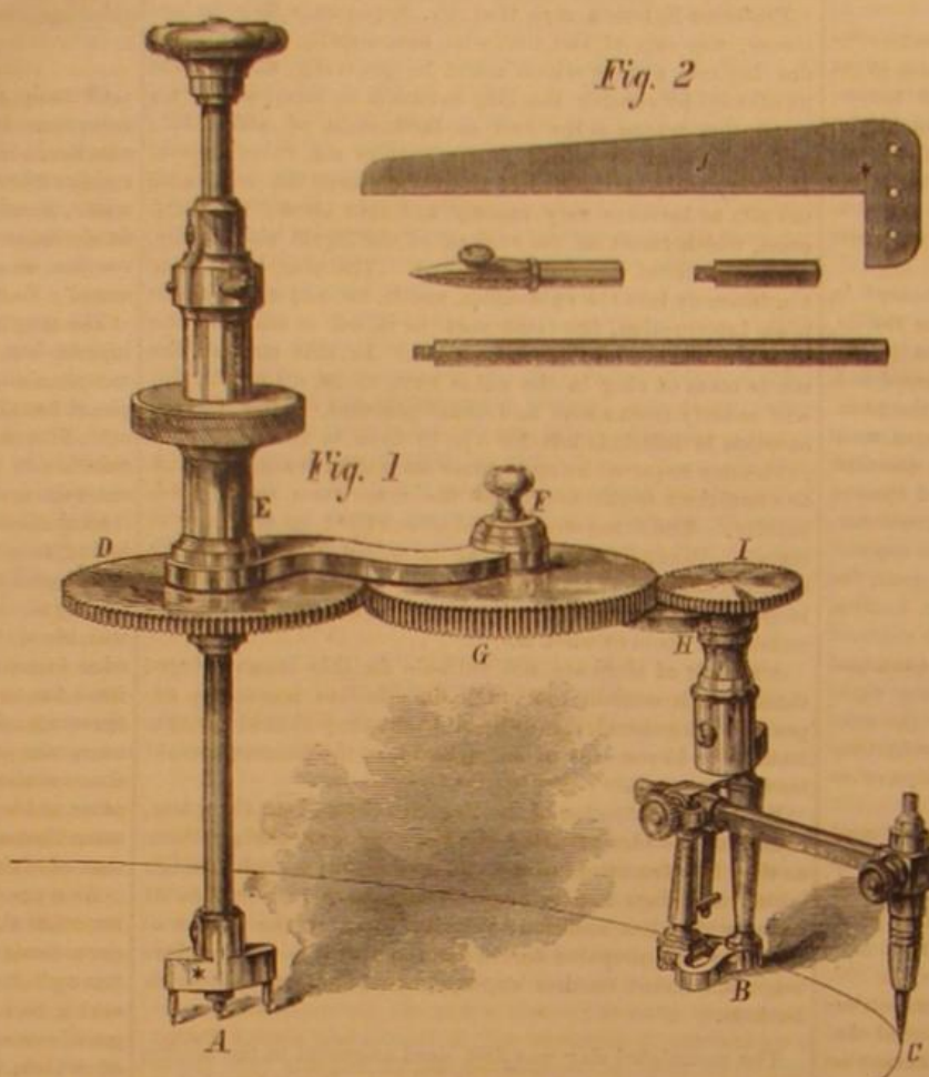
BROWNE'S ELLIPSOGRAPH.
