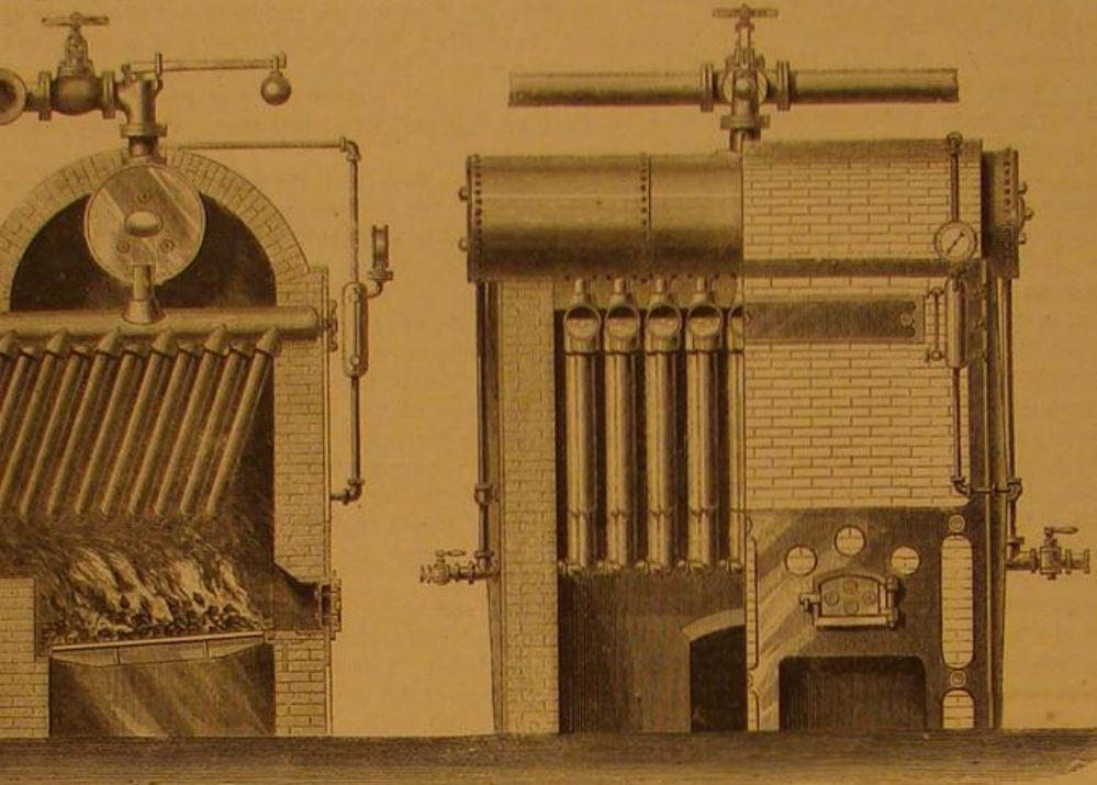
THE ALLEN STEAM BOILER.
